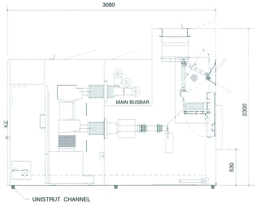
TYPICAL VH3 SECTIONAL VIEW
