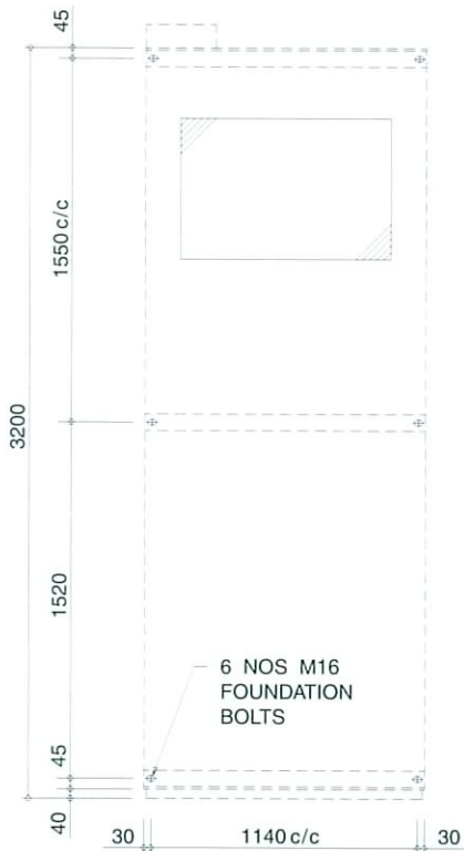
FOUNDATION PLAN
