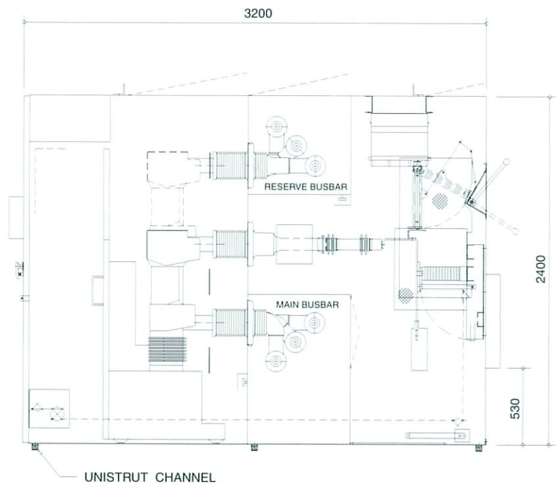
TYPICAL VH3D SECTIONAL VIEW
