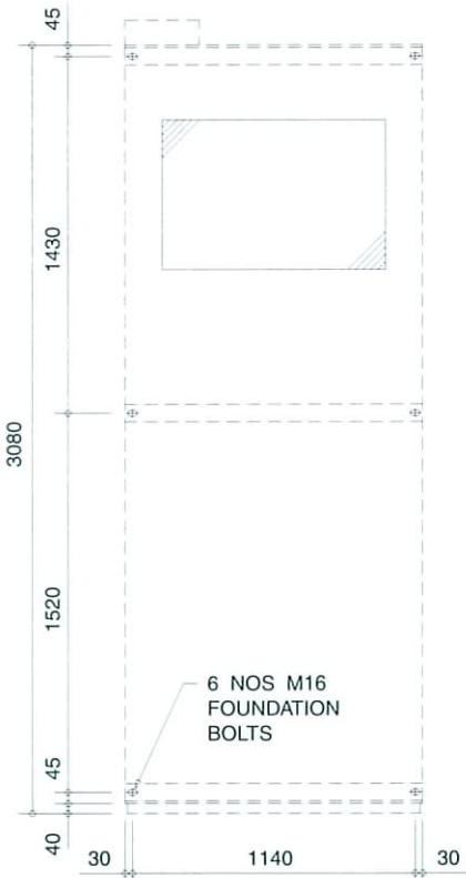
FOUNDATION PLAN
